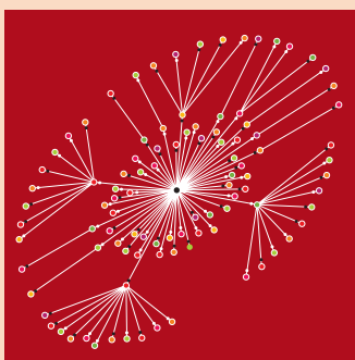
Image: Dynamical heterogeneities in granular media at the jamming transition (adapted from F Lechenault et al 2008 EPL 83 46003; artistic impression by Frédérique Swist).
